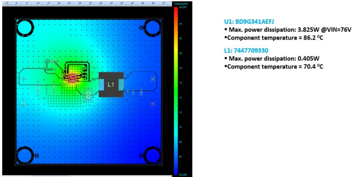
Fig 11: BD9G341AEFJ-E2EVK-101 Thermal Characteristics at Temp=25°C, No air flow, V_{IN}=76V , V_{OUT}=5V , I_{OUT}=3A . Thermal characteristics also apply to BD9G341AEFJ-EVK-101.
