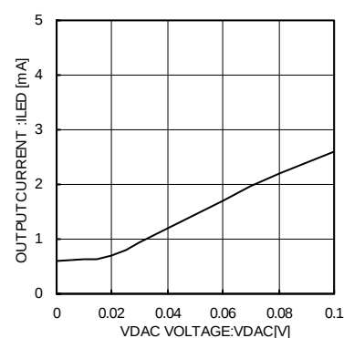
Fig.6 VDAC Gain②
