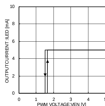
Fig.12 PWM threshold voltage
