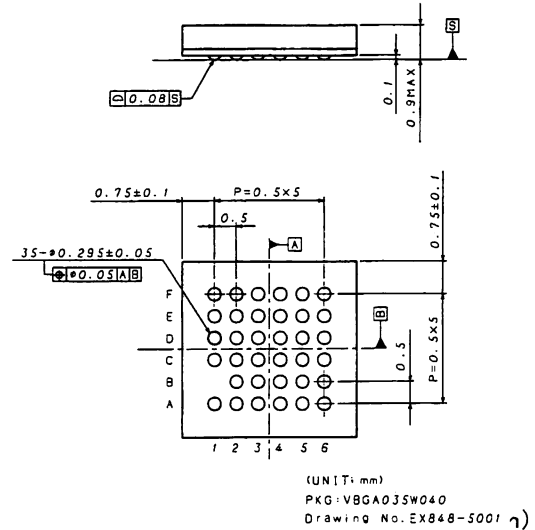
Figure 2 A terminal layout plan (Bottom view)
