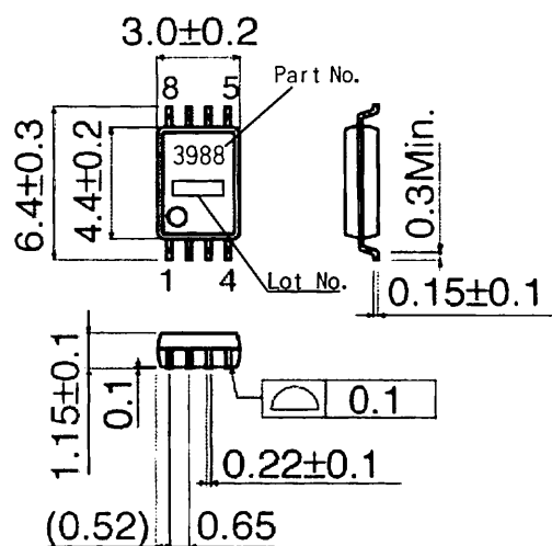
SS0P-B8 (UNIT : mm)
