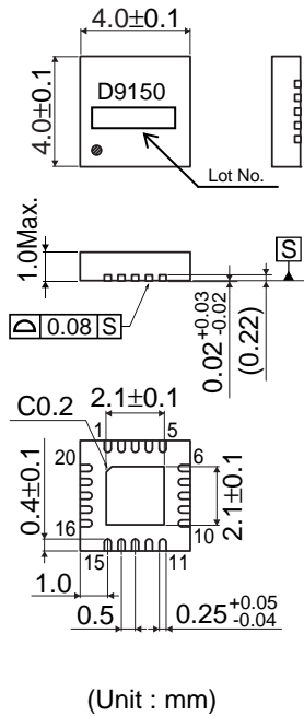
Fig.1 BD9150MUV TOP View
