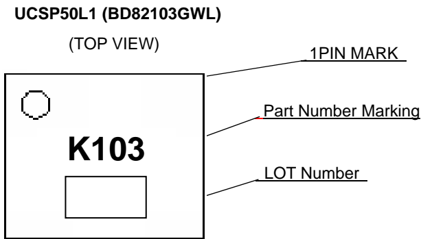
Figure 11. Marking Diagram
