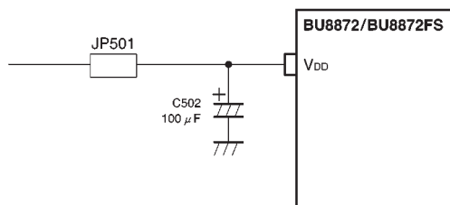
Fig. 5 Power supply circuit
