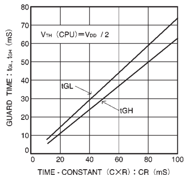
Fig. 9 Guard time vs. Time constant ( C \times R )
