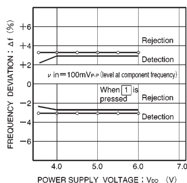
Fig. 13 Frequency detection/rejection ranges vs. power supply voltage
