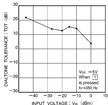
Fig. 16 Dial tone tolerance range vs. input voltage
