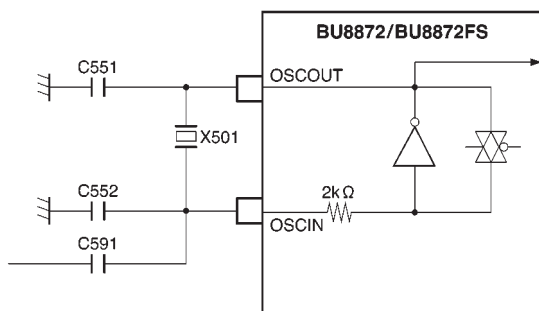
Fig. 6 Oscillation circuit
