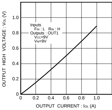
Fig.11 Output low level voltage vs. output current
