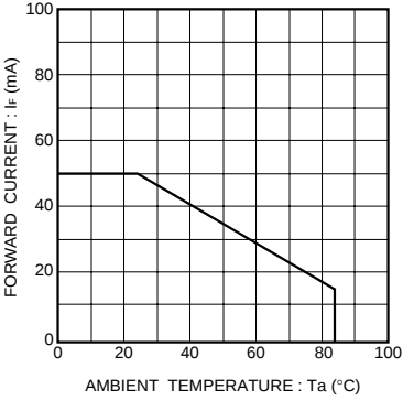
Fig.9 Forward current vs. ambient temperature
