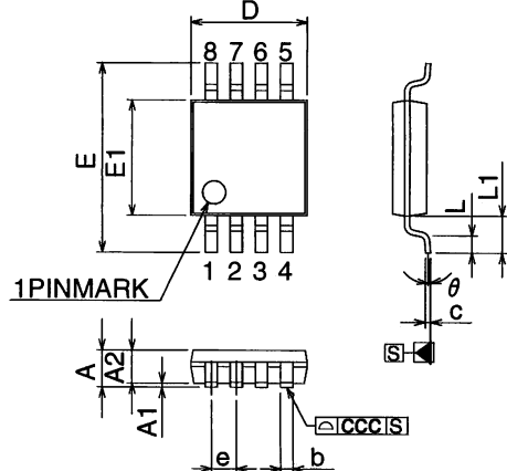
Fig.-4 TSSOP Package Outline
