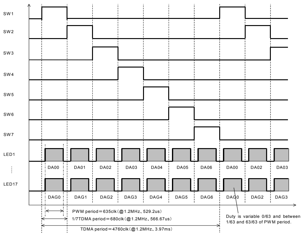
Fig.11 SW timing
