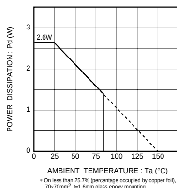
Fig.4 Power dissipation
