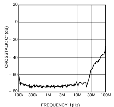
Fig. 4 Interchannel crosstalk
