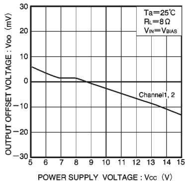
Fig. 4 Power supply voltage vs. output offset voltage
