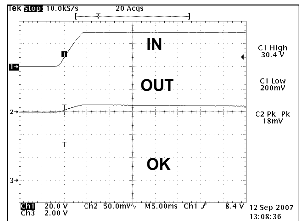
Figure 8. Input Steps (0→30V)
