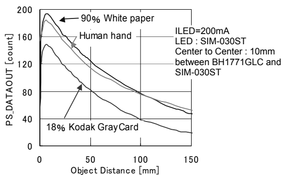
Fig.19 Object Distance – PS_DATAOUT of different objects
