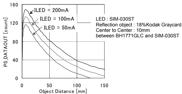
Fig.20 Object Distance – PS_DATAOUT of different ILED
