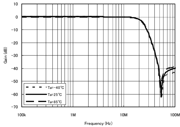
Fig.9 13.5MHzLPF Temp. - Freq. Characteristics
