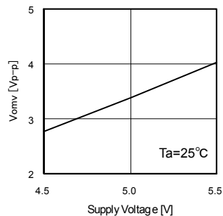
Fig.35 Vomv (PY-30MHz)
