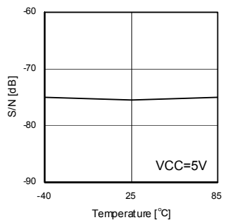
Fig.82 S/N(PY-13.5MHz)
