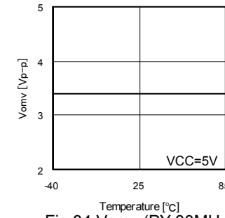
Fig.34 Vomv (PY-30MHz)
