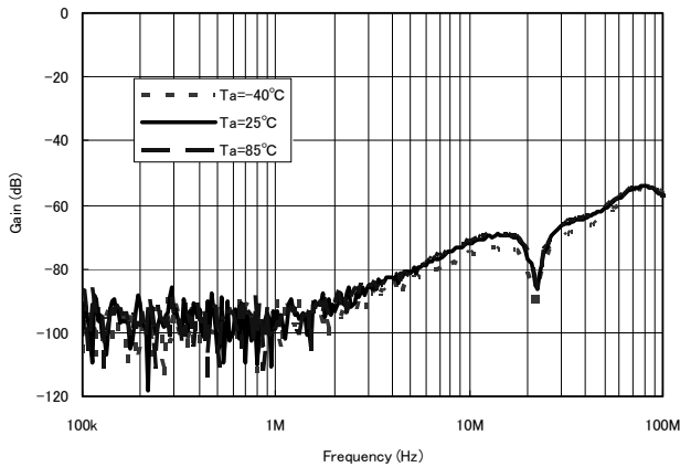
Fig.22 13.5MHzLPF Temp. - MUTE attenuation
