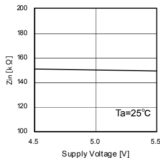
Fig.45 PB/PR_IN input impedance
