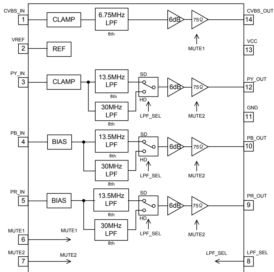
Fig.94 Block Diagram
