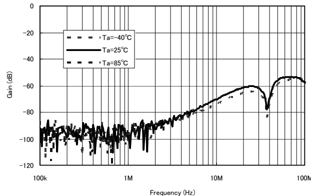
Fig.24 30MHzLPF Temp. - MUTE attenuation
