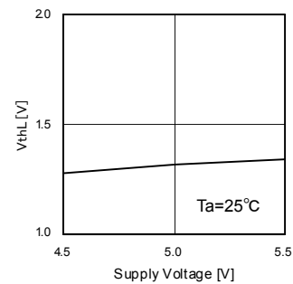
Fig.49 Control pin input voltage=L
