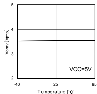
Fig.40 Vomv (PR-13.5MHz)
