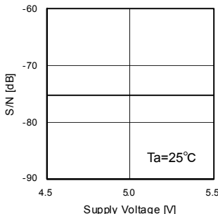
Fig.89 S/N (PB-30MHz)
