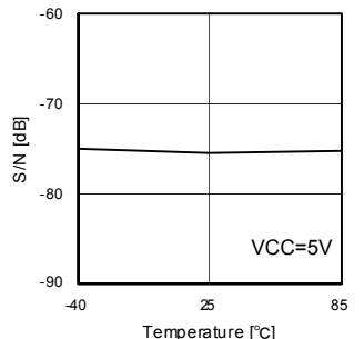
Fig.90 S/N (PR-13.5MHz)
