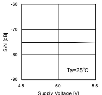
Fig.93 S/N (PR-30MHz)
