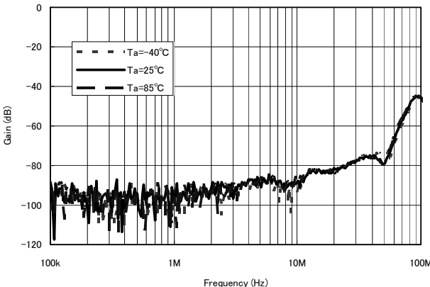
Fig.20 6.75MHzLPF Temp. - MUTE attenuation
