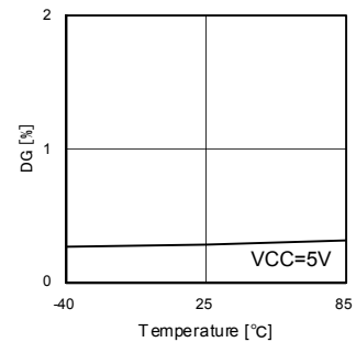
Fig.52DG(CVBS)
