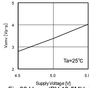
Fig.33 Vomv (PY-13.5MHz)
