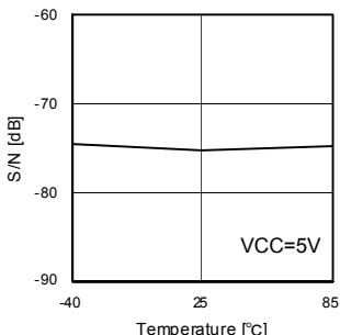
Fig.92 S/N (PR-30MHz)
