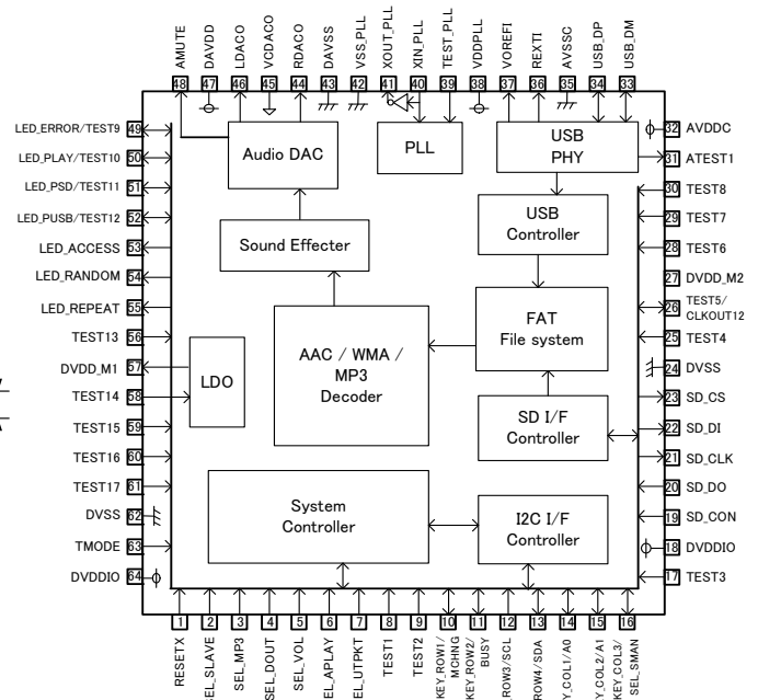
Figure 2. Block diagram
