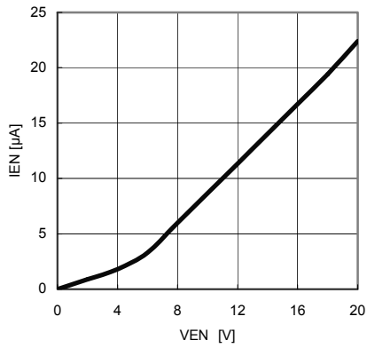
Fig.16 VEN-IEN
