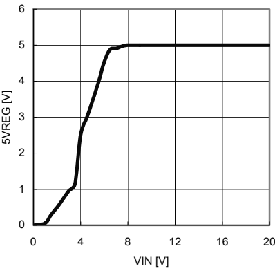
Fig.15 VIN-5VREG
