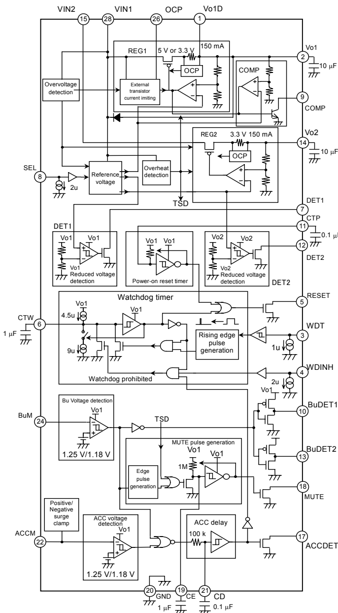
Fig.49 Block Diagram
