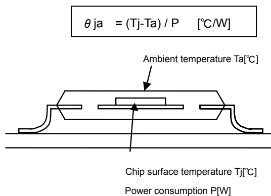
Fig.37 Thermal resistance
