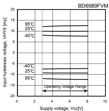
Fig.7 Input hysteresis voltage
