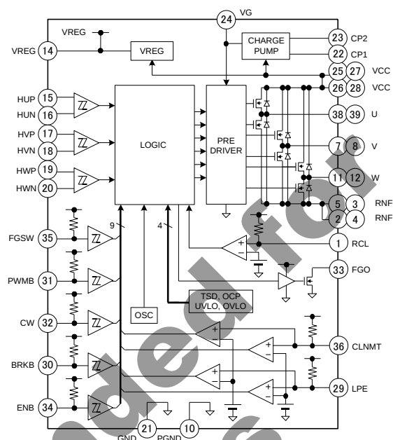
Figure 3. Block Diagram
