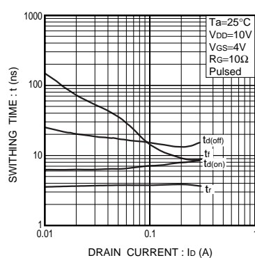
Fig.7 Switching characteristics
