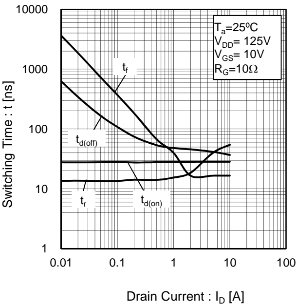
Fig.18 Switching Characteristics
