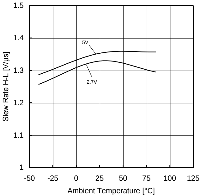
Figure 21. Slew Rate H-L vs Ambient Temperature ( R_L=10k\Omega )
