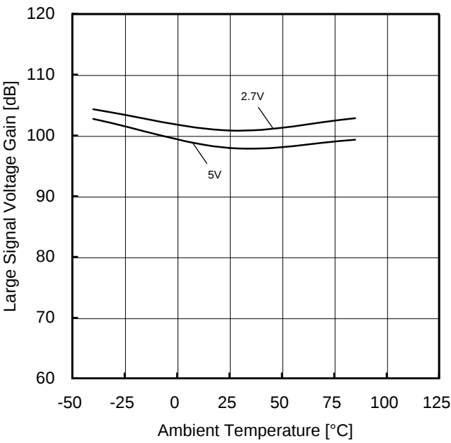
Figure 40. Large Signal Voltage Gain vs Ambient Temperature
