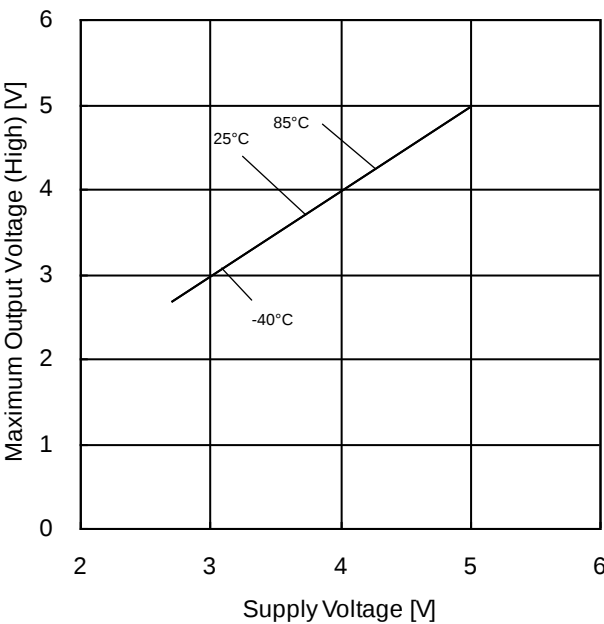
Figure 4. Maximum Output Voltage High vs Supply Voltage (RL=2kΩ)
