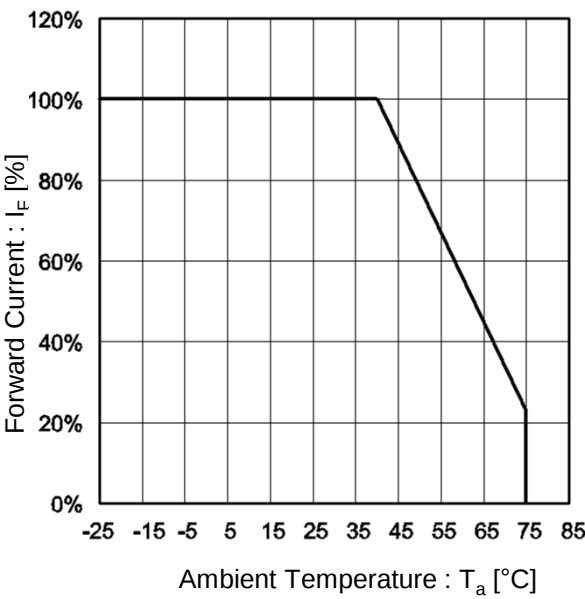
Fig.6 Derating
