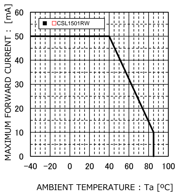
Fig.4 Derating
