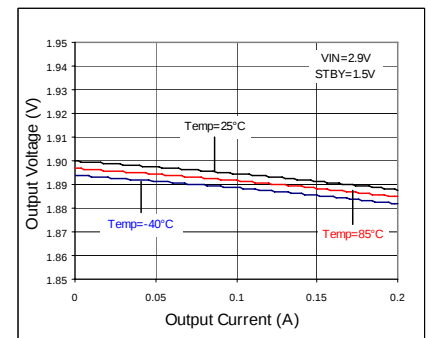
Fig 83. Load Regulation
