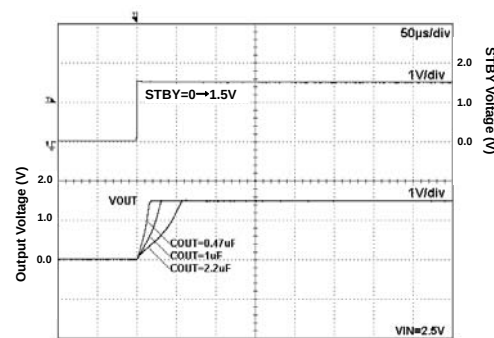
Fig 48. Start Up Time I_{out}=200\text{mA}
