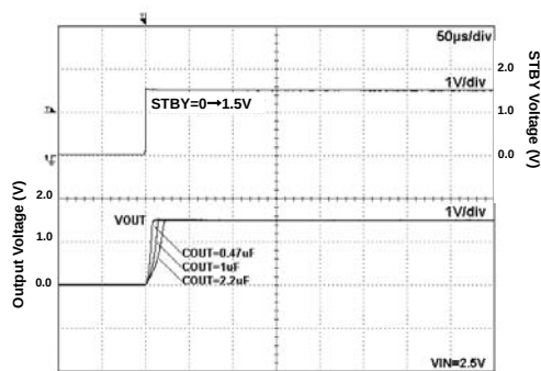
Fig 47. Start Up Time I_{out}=0\text{mA}
