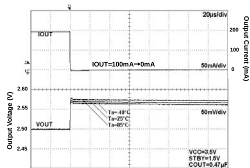
Fig 118. Load Response
