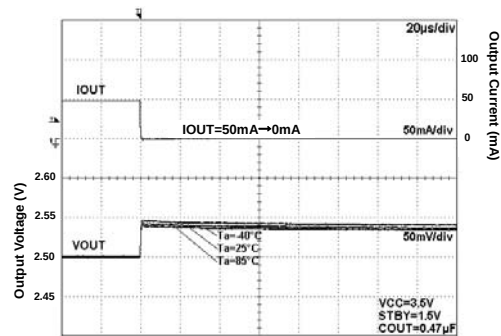
Fig 116. Load Response
