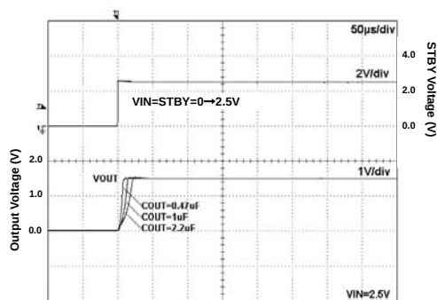
Fig 49. Start Up Time ( V_{IN}=STBY ) I_{out}=0\text{mA} I_{out}=0\text{mA}
