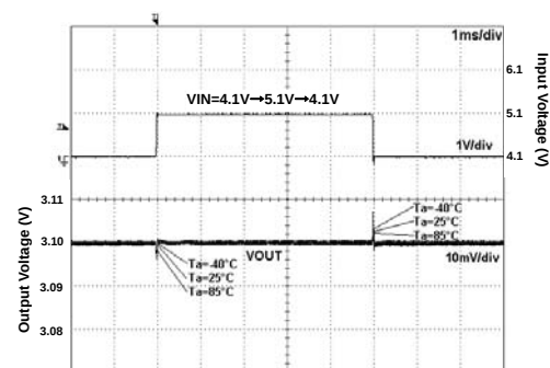
Fig 258. VIN Response
