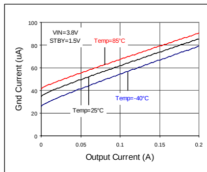
Fig 185. IOU - IGND
