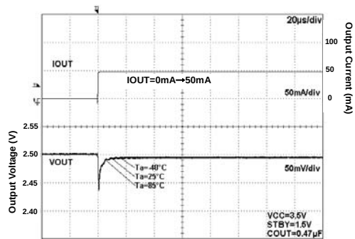
Fig 115. Load Response
