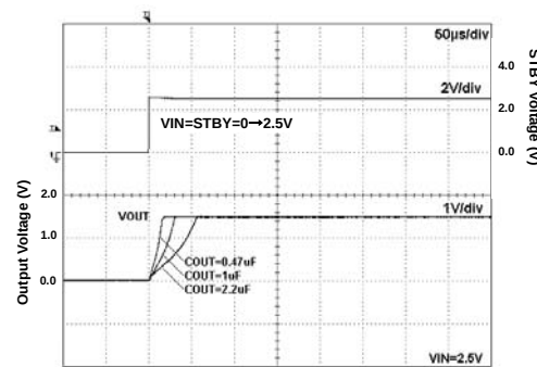
Fig 50. Start Up Time ( V_{IN}=STBY ) I_{out}=200\text{mA}
