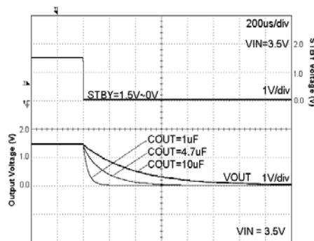
Fig. 32 Discharge Time Iout = 0 mA
