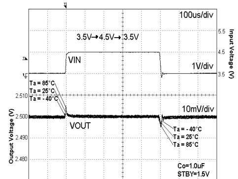
Fig. 91 VIN Response I_{out} = 10\text{mA}
