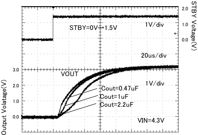
Figure 19. Startup time ( Rout = none )
