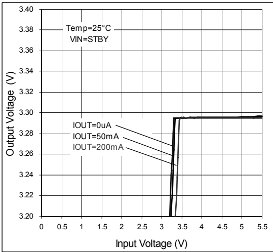
Figure 4. Line Regulation
