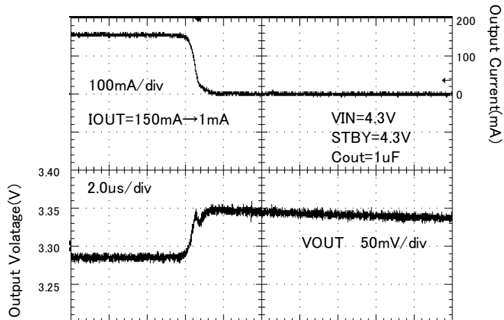
Figure 24. Load response ( I_{out} = 150\text{mA} \rightarrow 1\text{mA} )
