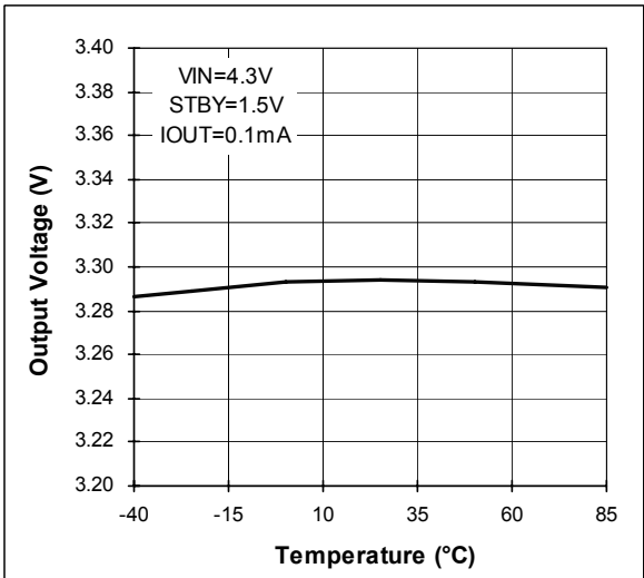
Figure 9. Output Voltage vs. Temperature
