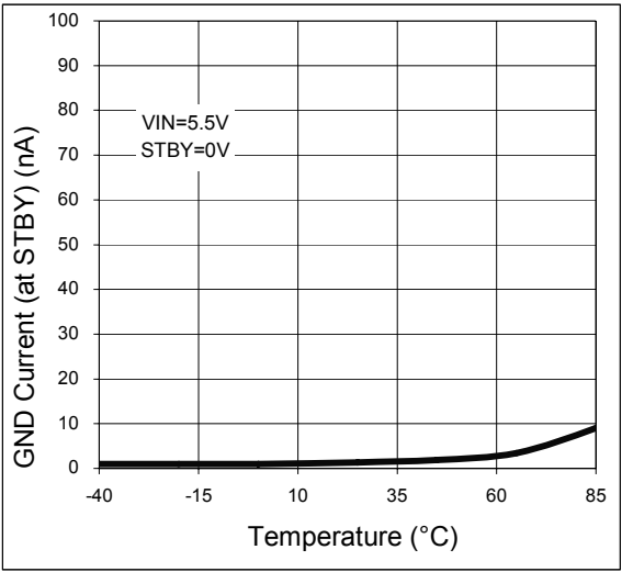
Figure 12. GND Current (at STBY) vs. Temperature
