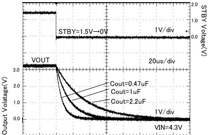
Figure 22. Discharge time ( Rout = 16.5 ohm )
