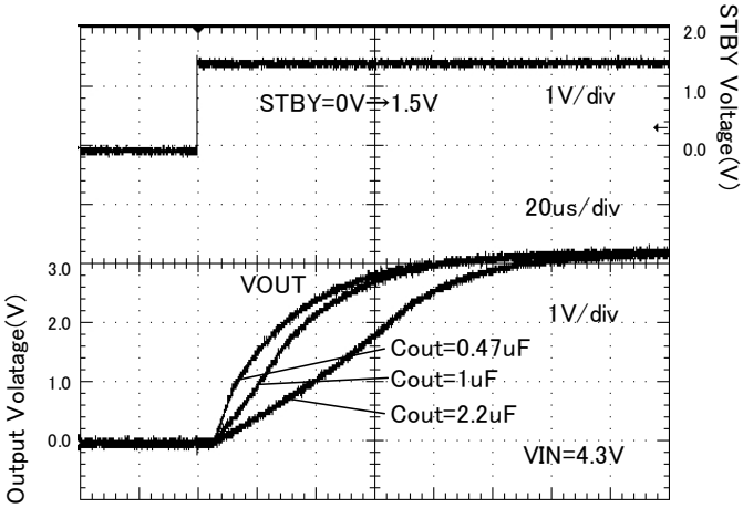
Figure 20. Startup time ( Rout = 16.5 ohm )
