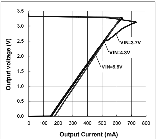
Figure 8. OCP Threshold
