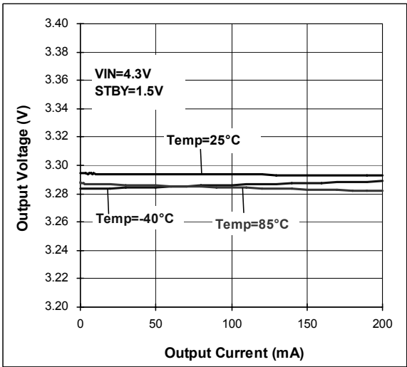
Figure 6. Load Regulation
