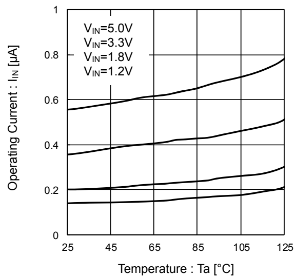
Figure 9. Operating Current vs Temperature
