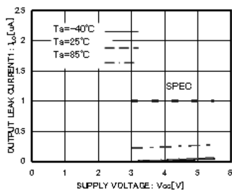
Figure 18. OUTPUT LEAK CURRENT I_{LO0} (SDA0 to 3)
