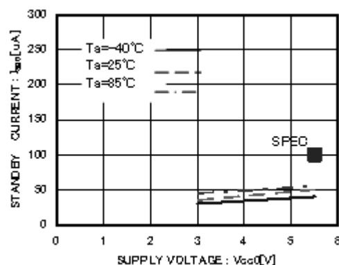
Figure 21. Standby Current I_{SB0}
