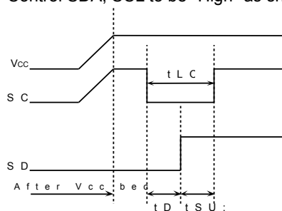
Figure 18. SCL="L" and SDA="L"
