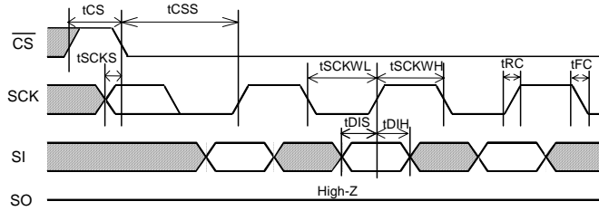
Figure 1. Input timing
