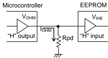
Figure 49. Input terminals Pull down resistance
