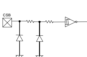
Figure 45. CSB terminals equivalent circuit
