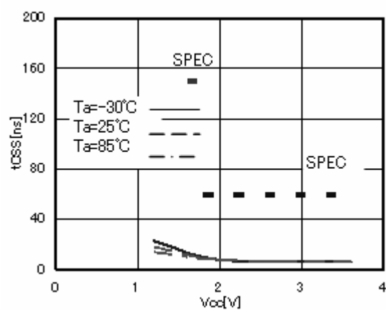
Figure 18. CSB setup time t_{CSS}
