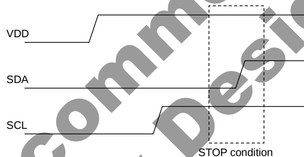
Figure 13. STOP condition
