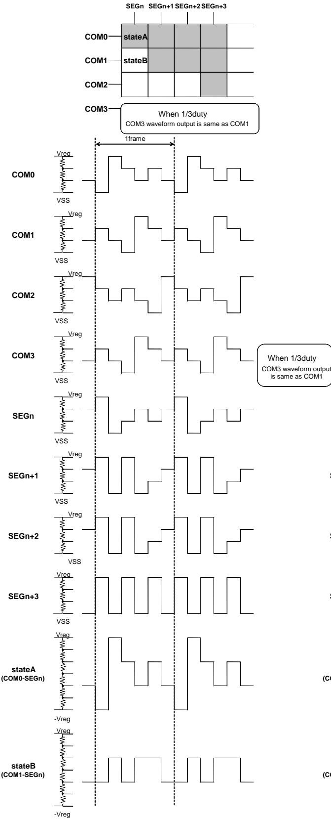
Figure 11. LCD Drive Waveform during Line inversion
