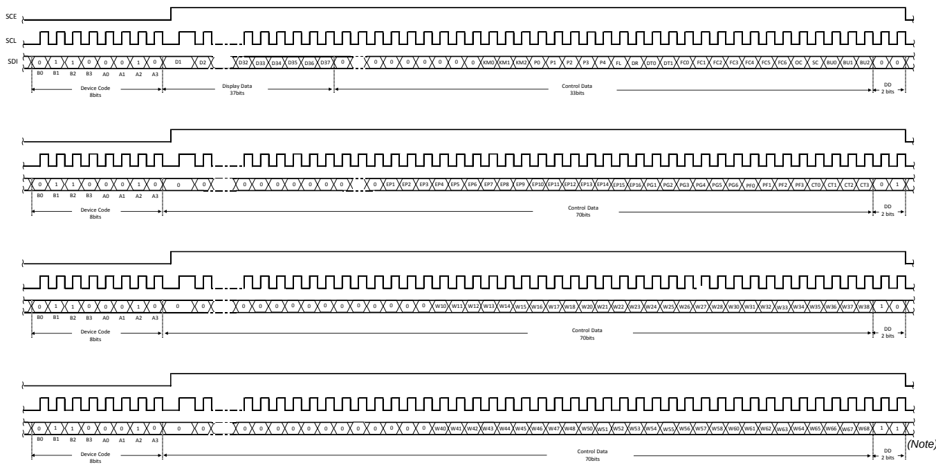
Figure 13. 3-SPI Data Transfer Format
