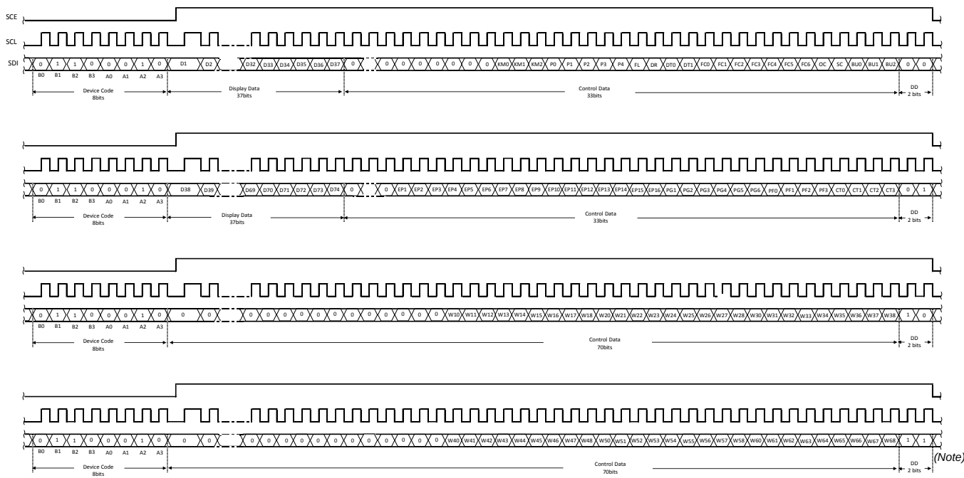
Figure 11. 3-SPI Data Transfer Format
