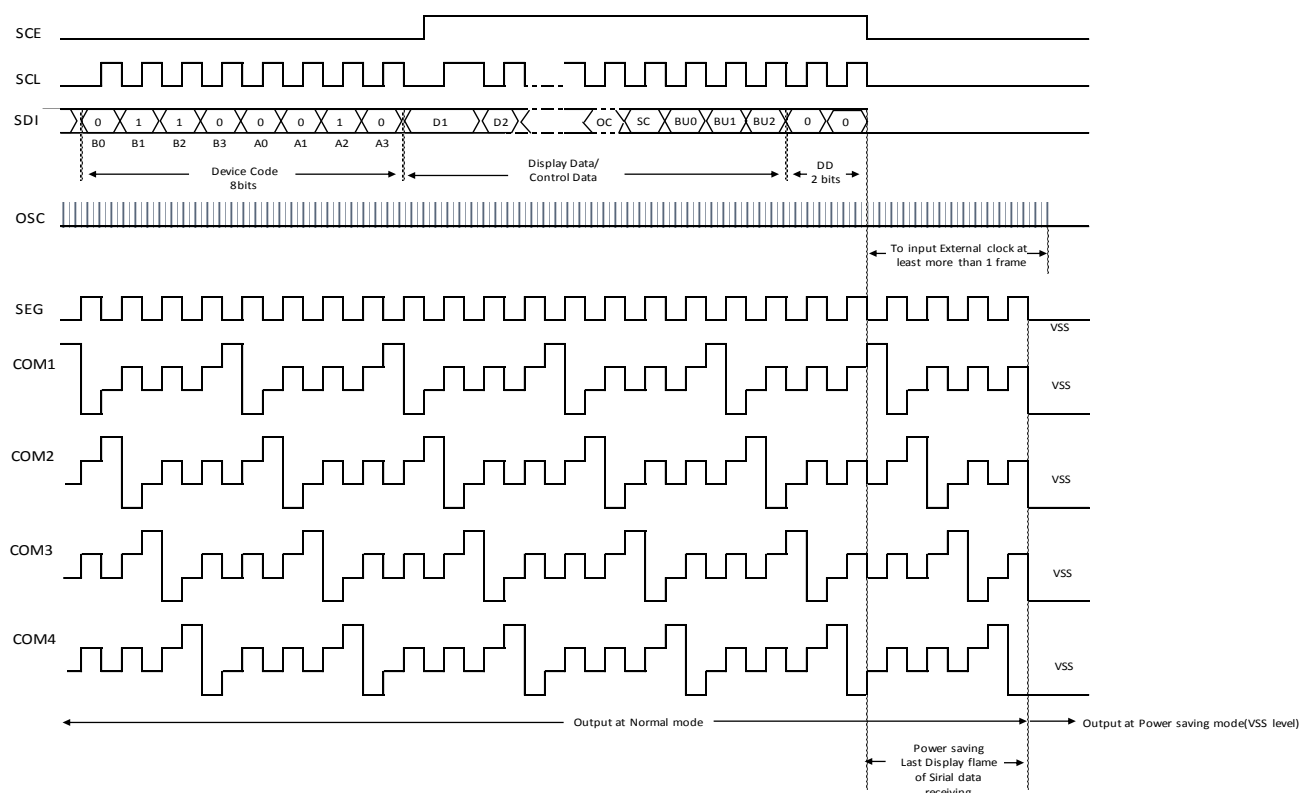
Figure 43. External Stop Timing(1/4-Duty)
