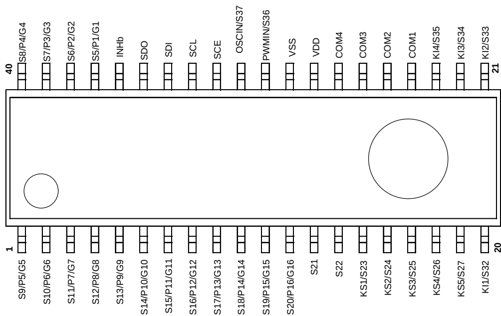
Figure 3. Pin Configuration (TOP VIEW)
