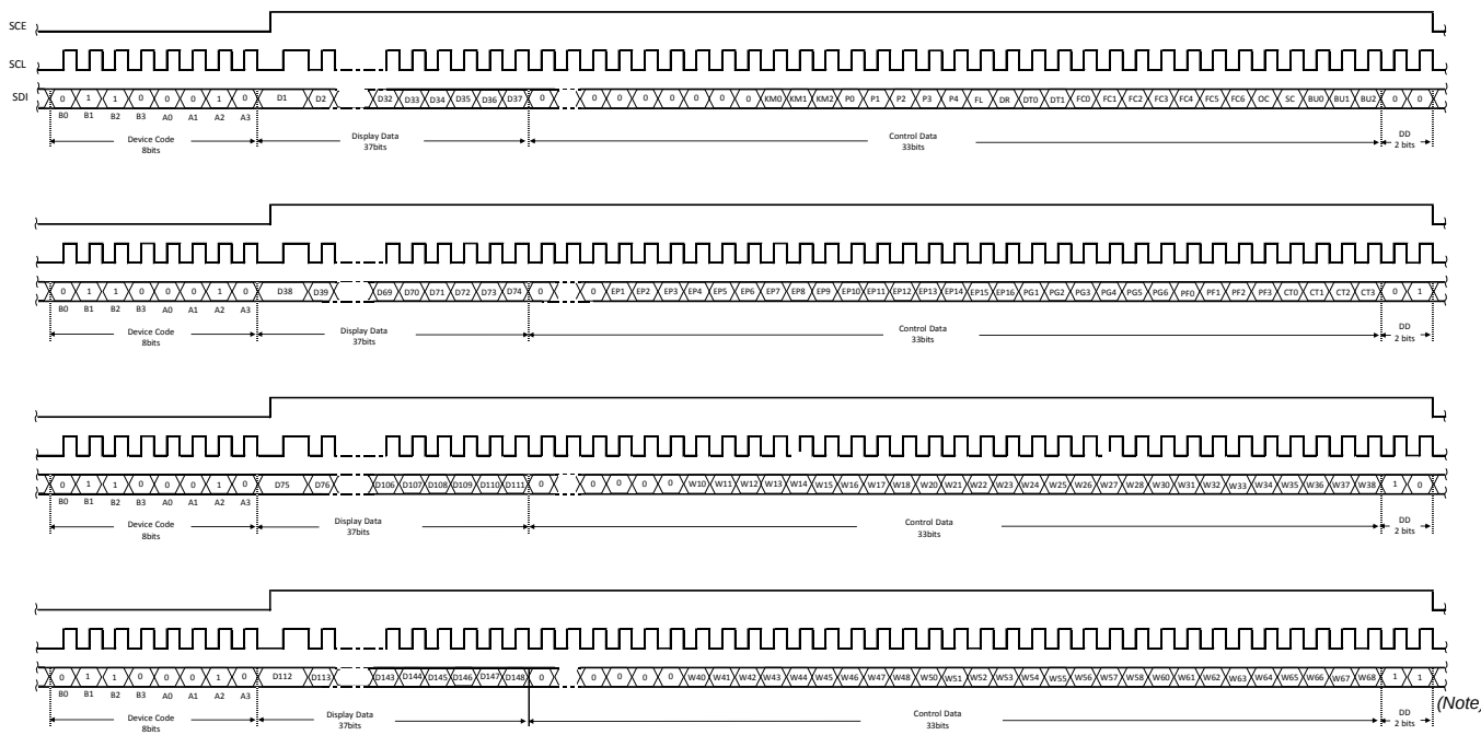
Figure 7. 3-SPI Data Transfer Format
