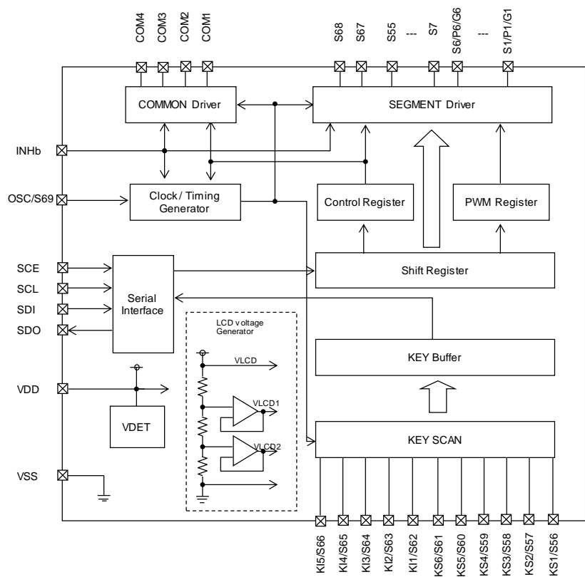
Figure 2. Block Diagram
