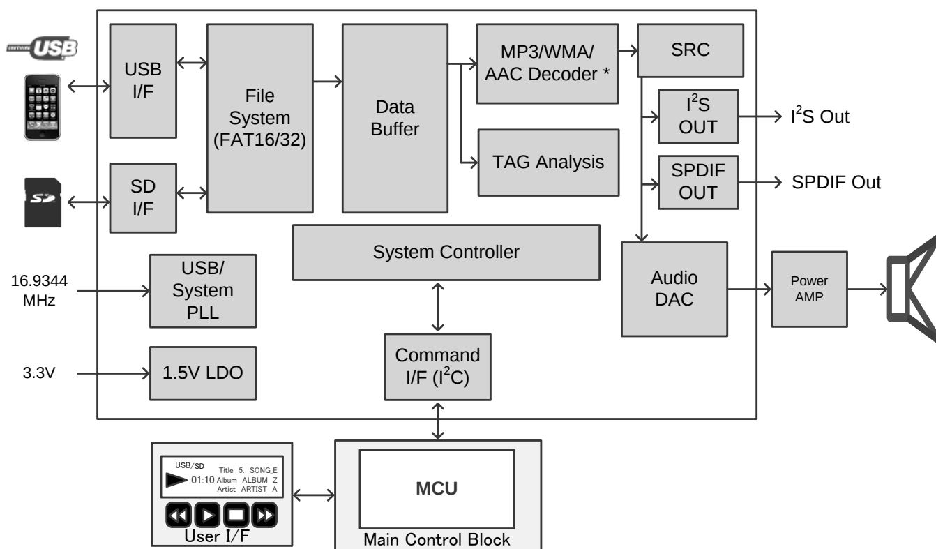
Figure 4. Block diagram
