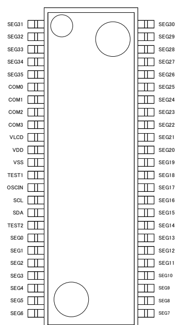
Figure 5. Pin Configuration (TOP VIEW)
