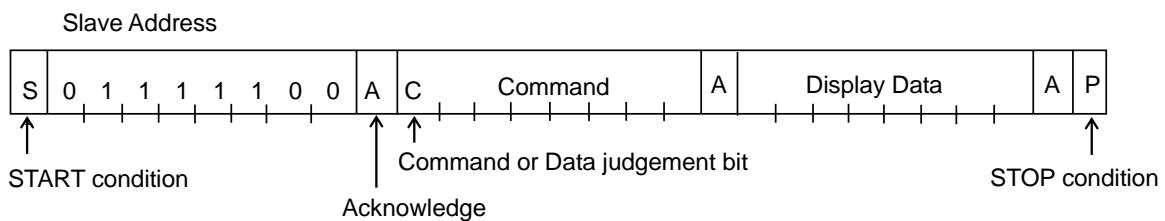
Figure 9. Interface Protocol
