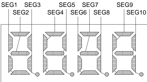
Figure 14. Example SEG Line Pattern
