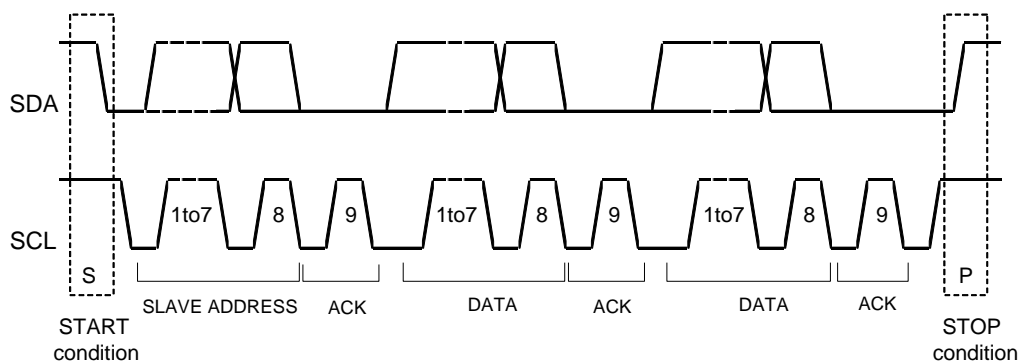
Figure 7. Acknowledge Timing
