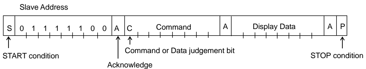
Figure 6. Interface Protocol
