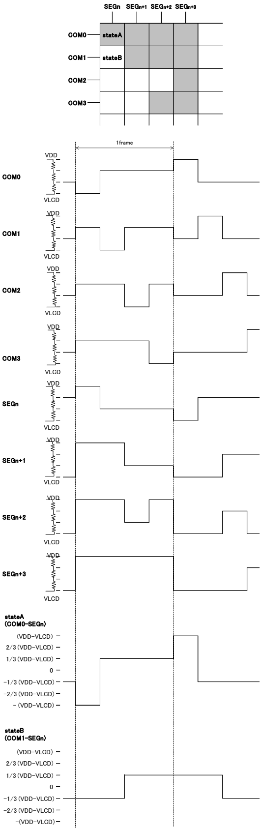
Figure 12. LCD Waveform at Frame Inversion (1/3bias)
