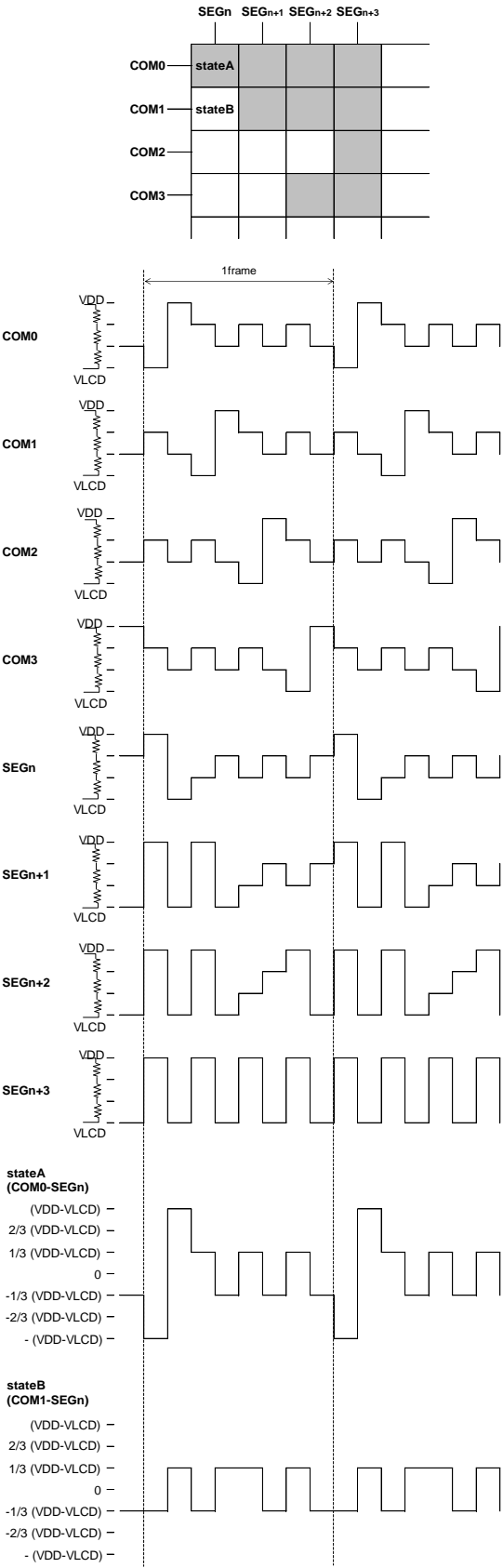
Figure 11. LCD Waveform at Line Inversion (1/3bias)
