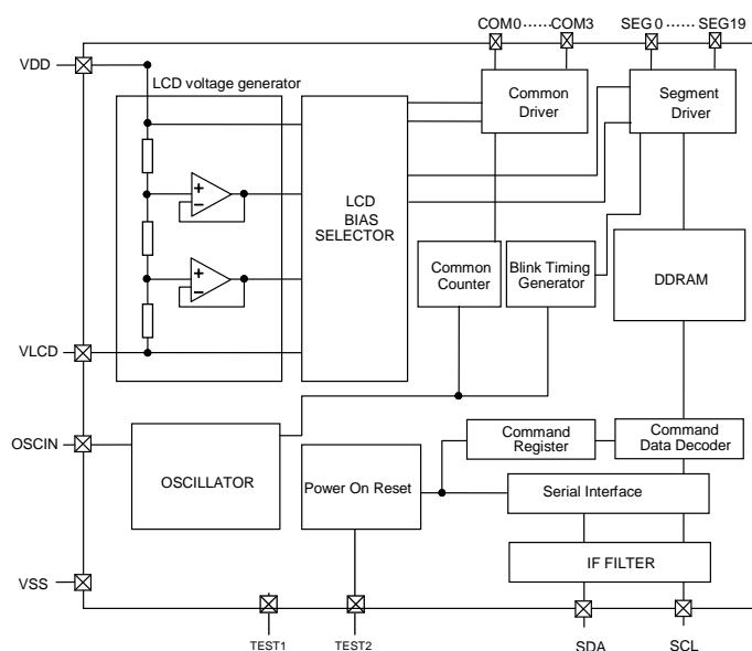
Figure 1. Block Diagram
