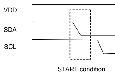
Figure 19. START Condition
