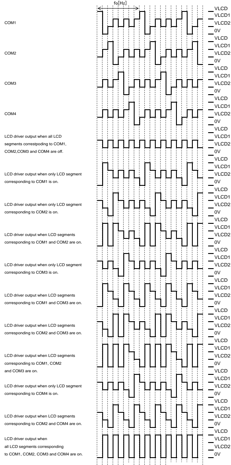
Figure 11. LCD Waveform (1/4 Duty, 1/3 Bias)
