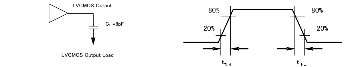
Figure 6. LVC MOS Output Load and Transition Time
