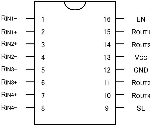
Fig.3. Pin Diagram (Top View)
