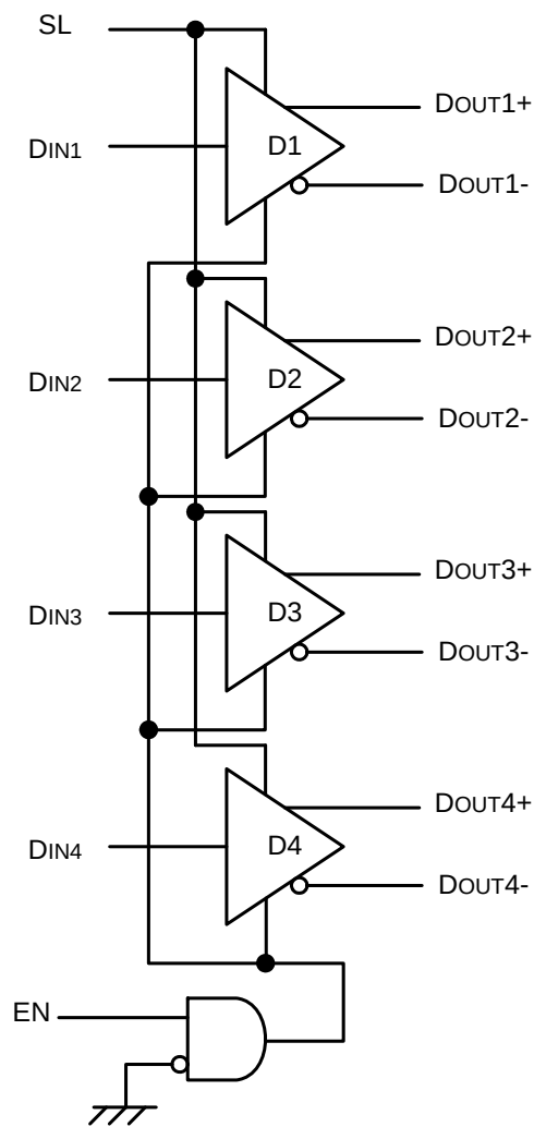
Fig.1. Block Diagram
