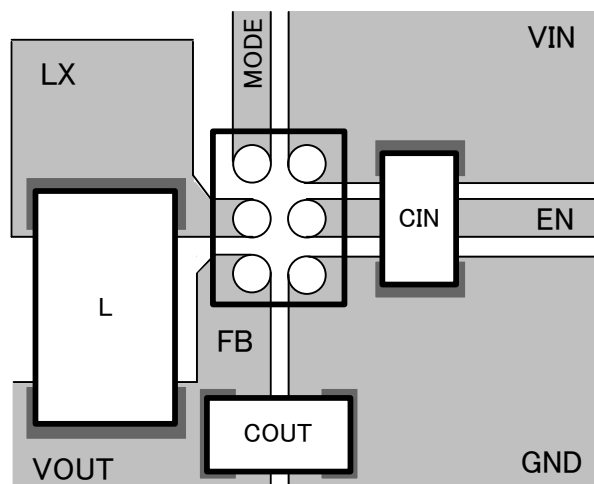
Figure 19. PCB layout
