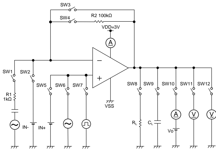
Figure 49. Test Circuit 2
